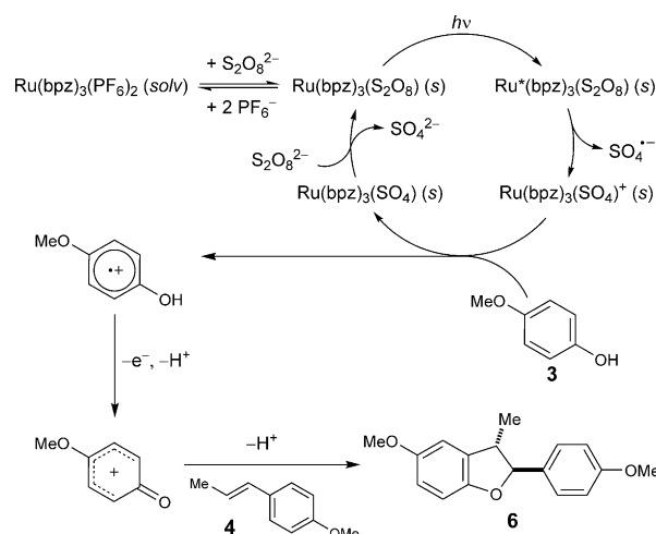
Scheme 2. Proposed mechanism for the oxidative [3+2] cycloaddition of phenols using \text{Ru}(\text{bpz})_3^{2+} .
